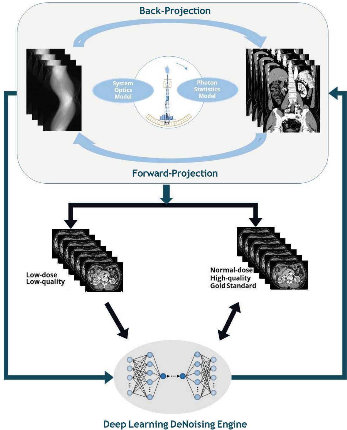
Figure 2. Deep Learning De-Noising Engine Training Process
