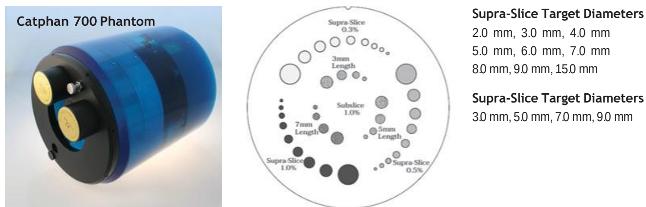
Figure 7a. Catphan 700 Phantom Includes Low-Contrast Module with Different Supra-Slice and Subslice Contrast Targets
